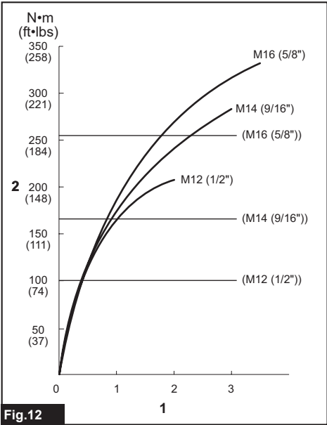
Fig.12 ► 1. Fastening time (seconds) 2. Fastening torque
