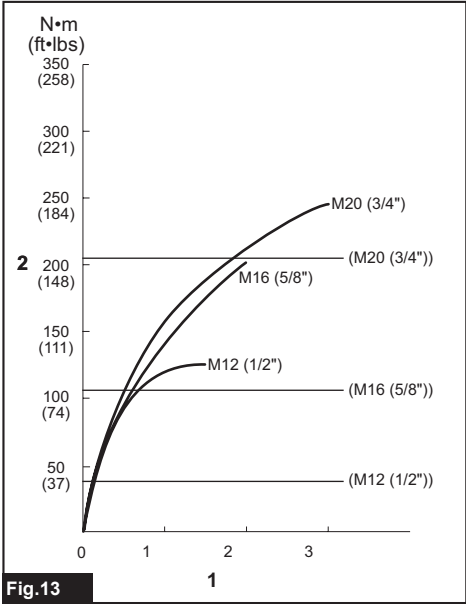
Fig.13 ► 1. Fastening time (seconds) 2. Fastening torque
