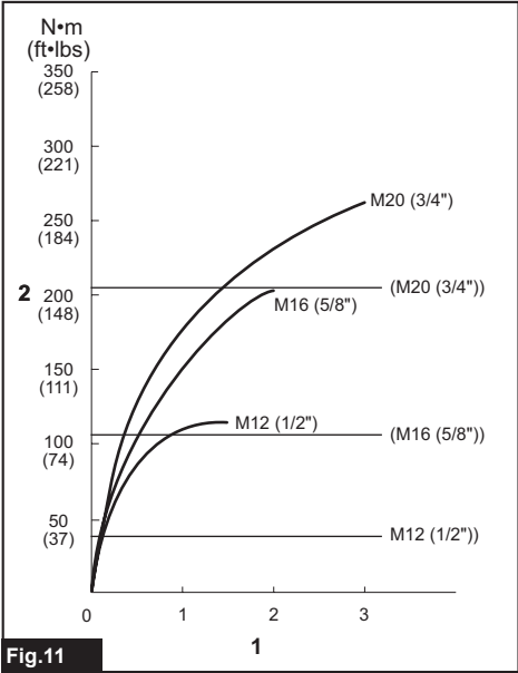
Fig.11 ► 1. Fastening time (seconds) 2. Fastening torque
