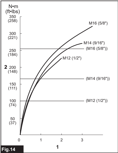
Fig.14 ► 1. Fastening time (seconds) 2. Fastening torque
